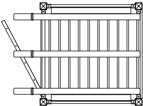
Single Model Top View N.T.S.
